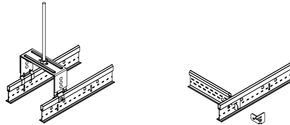
Service integration hanger bracket
