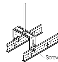
Service integration hanger bracket
