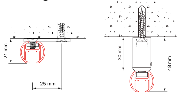
Ceilingmounting 4200 with ceiling bracket 5153
