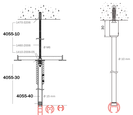
Ceiling mounting 4100, 5100 or 4200: threaded rod set 4055-10, suspension hanger tube 4055-40 and with fixing set 4055-30.
