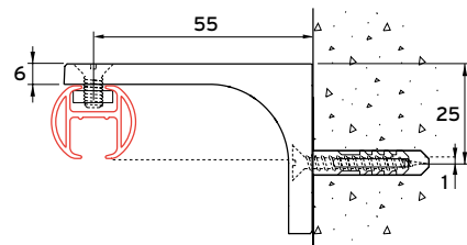
Mounting 4200 with wall bracket 5140
