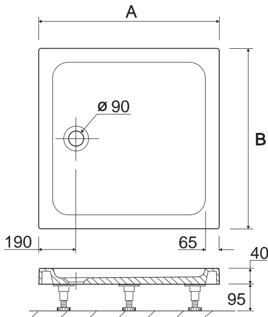
Square flat top tray
