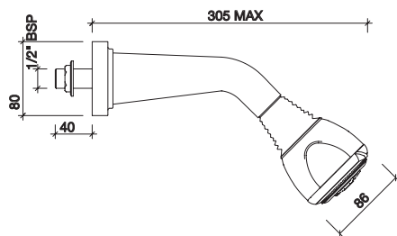
sola shower fixed head
