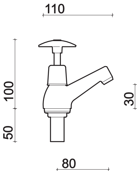
Cross head pillar taps
