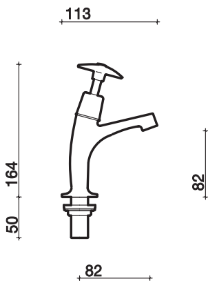
High neck cross head pillar taps
