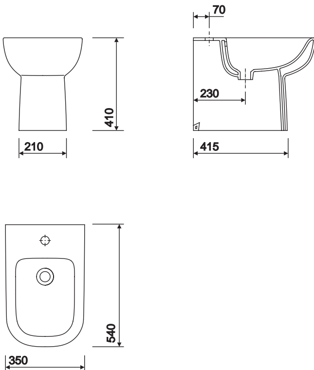
E500 floorstanding bidet
