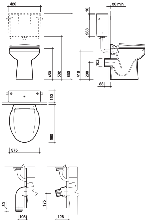
Avalon back-to-wall WC suite
