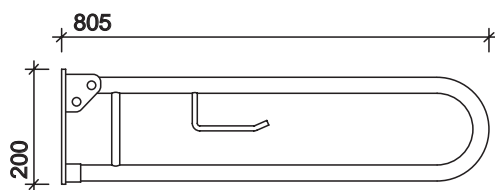
Hinged support rail with toilet roll holder
