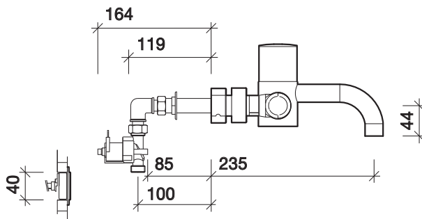
Cable to Battery 820mm Cable to Solenoid 1020mm
