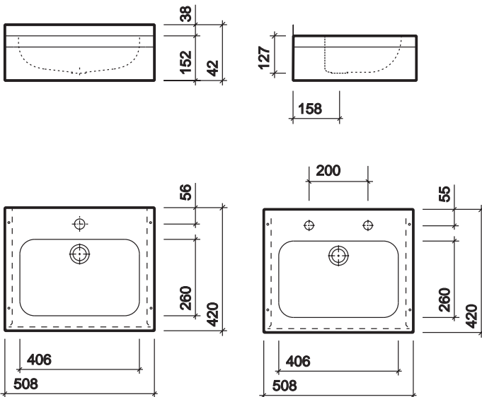
Wall hung basin 500 with apron
