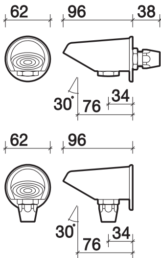
sola shower vandal resistant head
