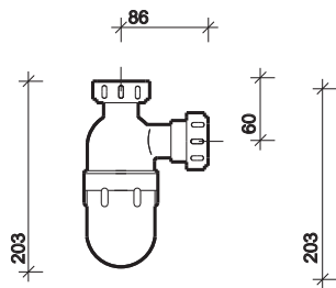
Acid proof bottle trap
