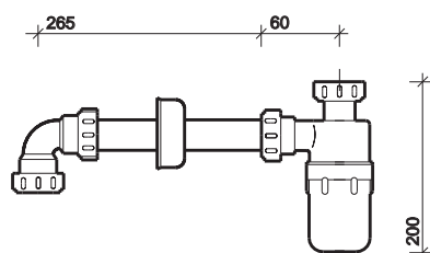
Resealing bottle trap
