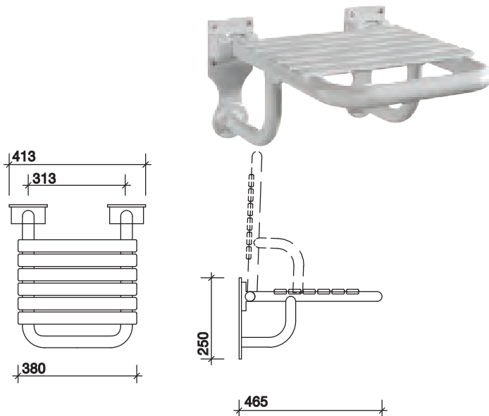
Shower seat
