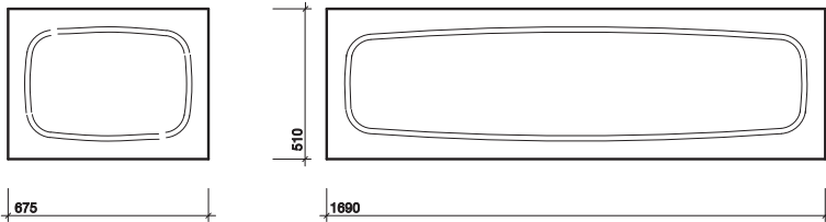
Refresh with Total Install® bath panels
