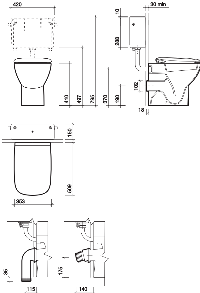
Moda back-to-wall washdown WC suite, horizontal outlet
