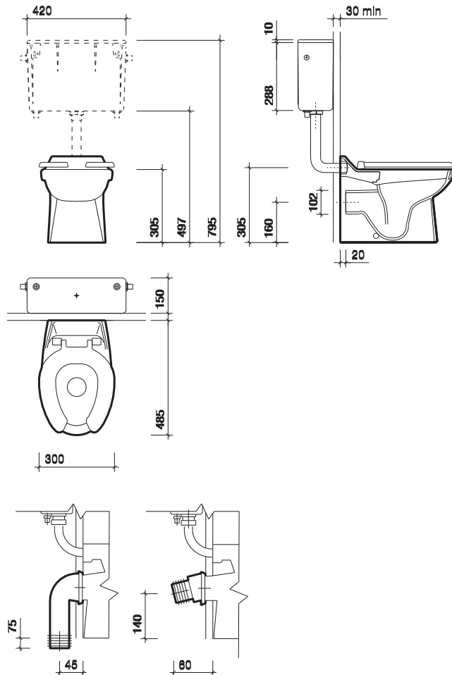
Sola school rimless 300 back-to-wall washdown WC suite
