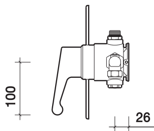
sola thermostatic shower valve - concealed
