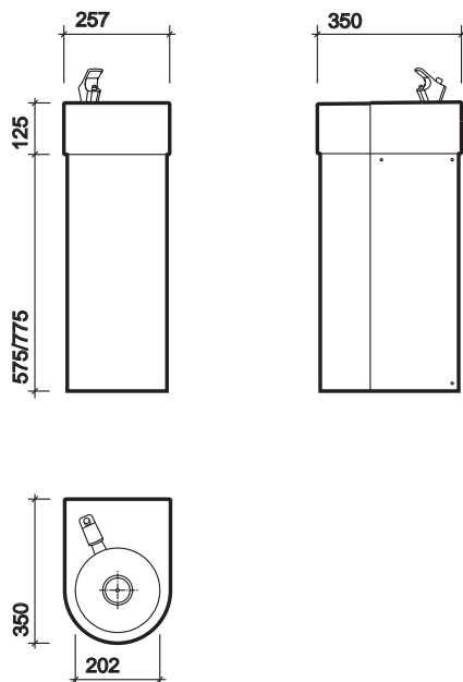
Drinking fountain - floor mounted (junior illustrated)
