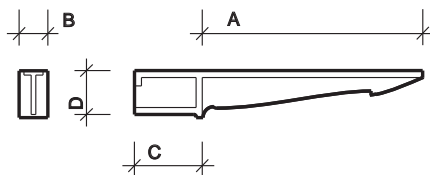
Build-in bracket
