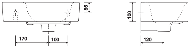
E200 400 x 250mm washbasin, with 1 RH Tap
