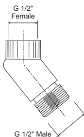
Shower hose angled connector 1/2" BSP
