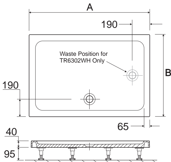
Rectangle flat top tray
