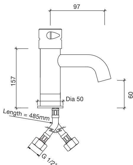
Non-concussive monobloc
