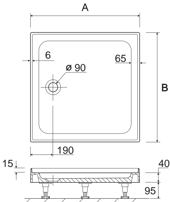
Square upstand tray
