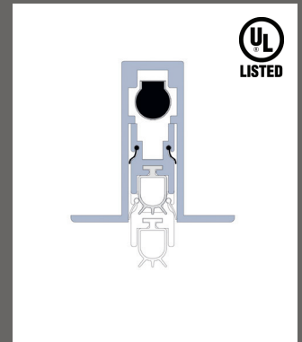
47730/A/B/C Automatic bottom door seal. Finishes: XX
