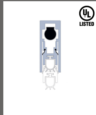
47720/A/B/C Automatic bottom door seal. Finishes: XX
